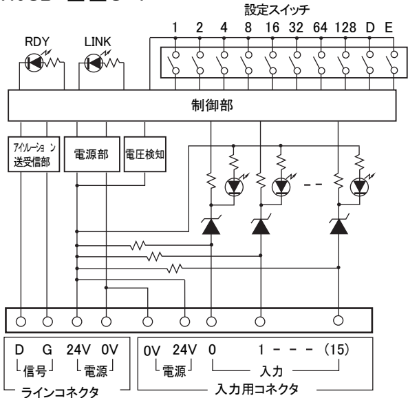
A49SB-□□U-4
