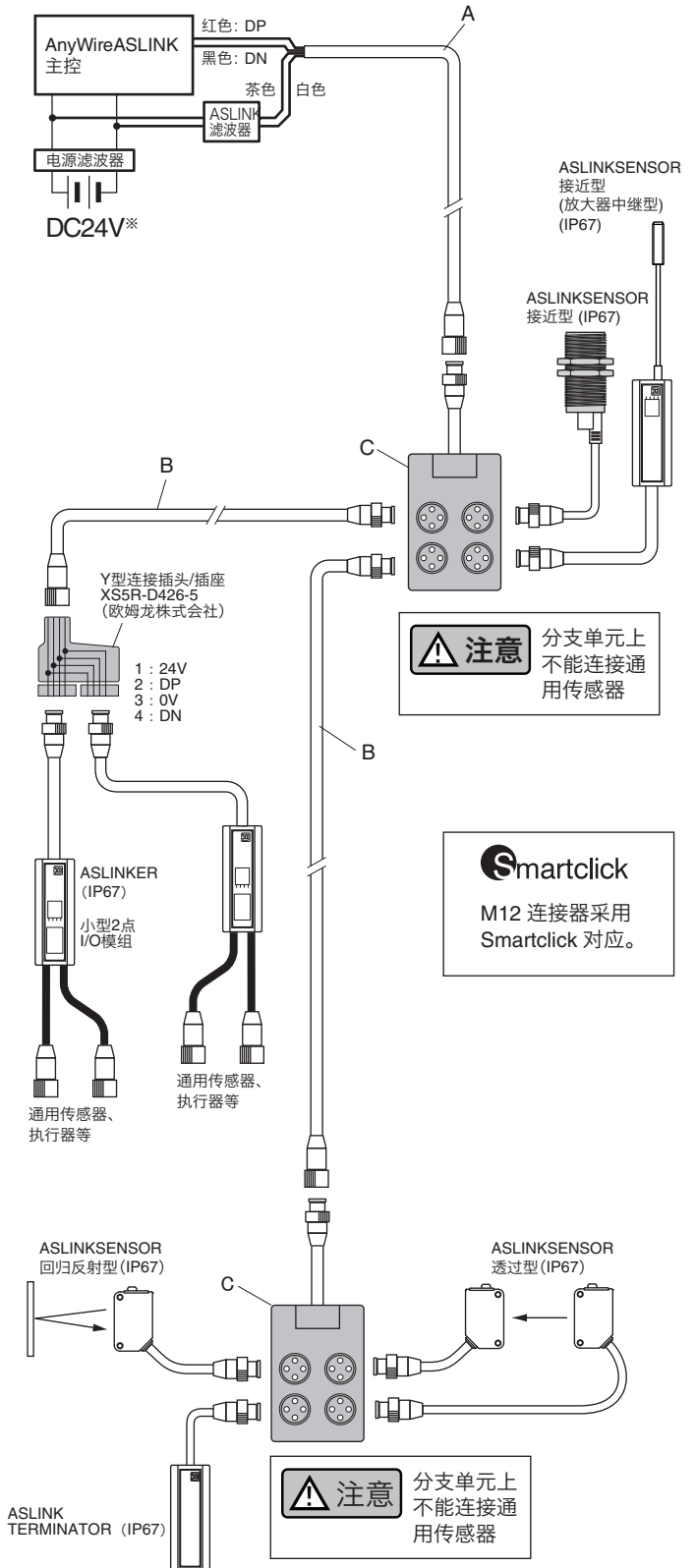
A 防水主线电缆 (1.25mm 2 )
